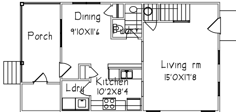
First Flr 704 sqft
